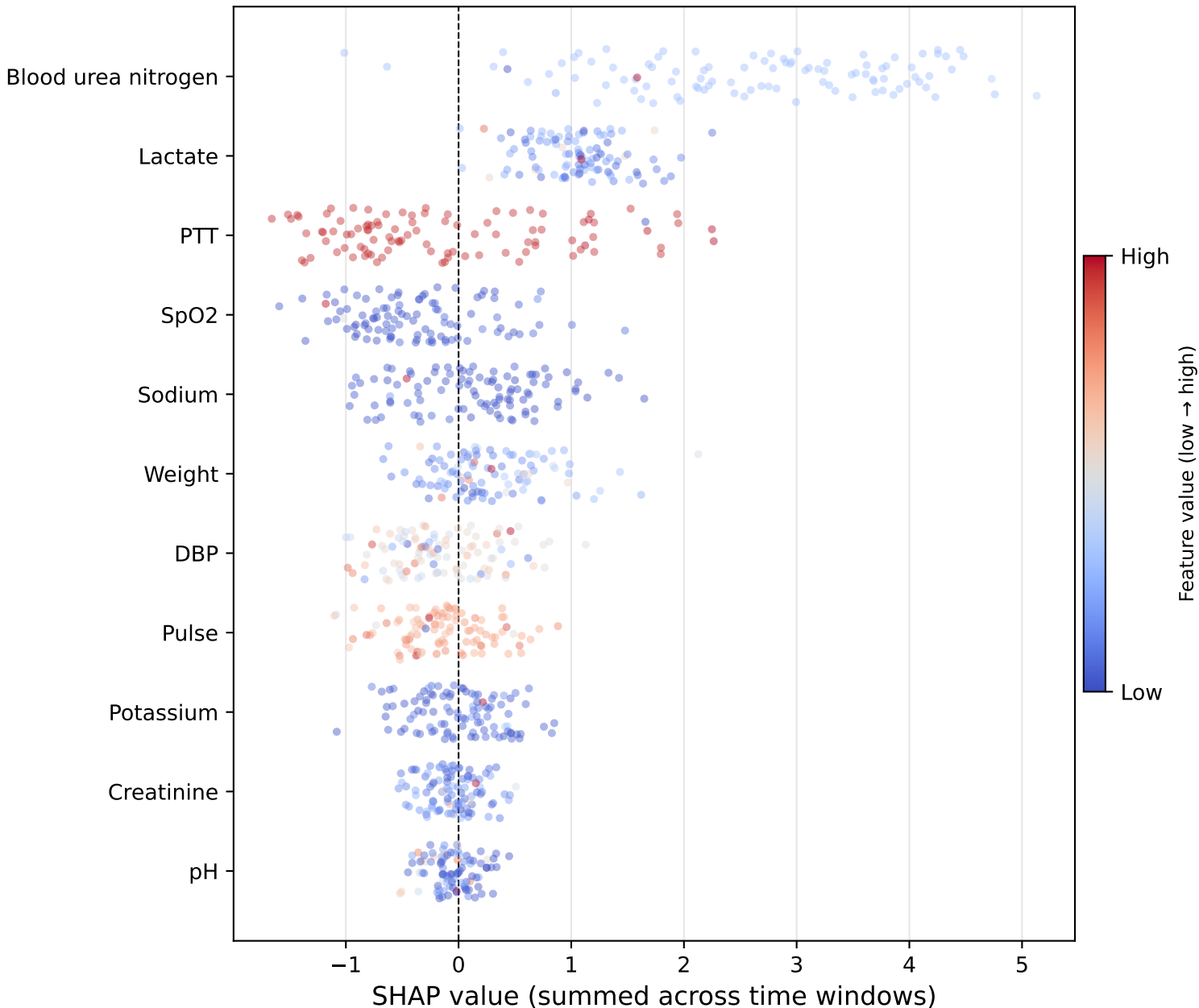
SHAP beeswarm — Simplified Clinician Consensus u Simplified Golem
